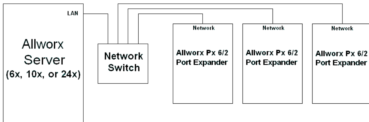
Figure 4, Connection Diagram
